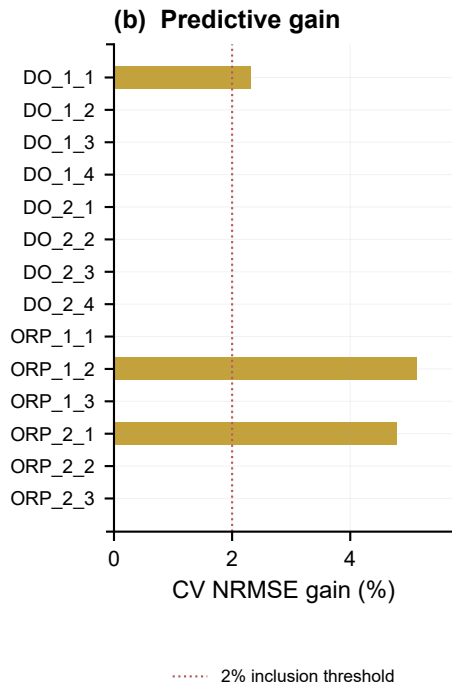
Figure 11. Same-analyte PLS peer selection with blocked temporal validation
