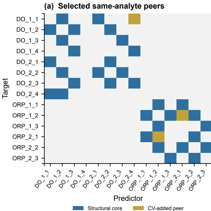
Figure 11. Same-analyte PLS peer selection with blocked temporal validation
